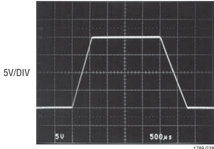
Large-Signal Transient Response G = 1, 10, 100
