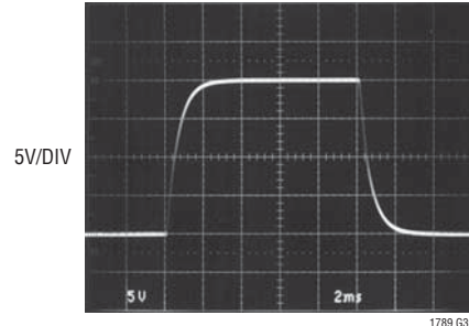
Large-Signal Transient Response G = 1000
