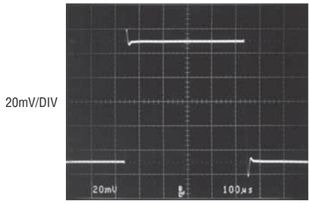
Small-Signal Transient Response G = 1
